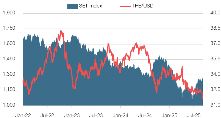
Fig 1: SET Index vs THB/USD
