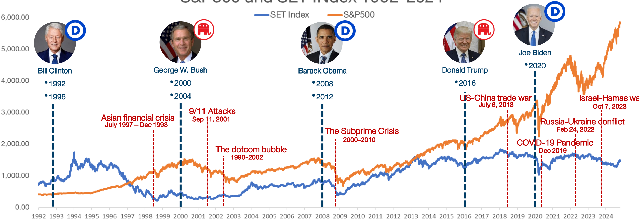
S&P500 and SET INdex 1992-2024
