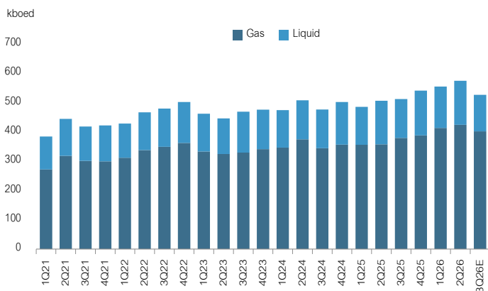
Fig 2: Quarterly average sales volume forecast
