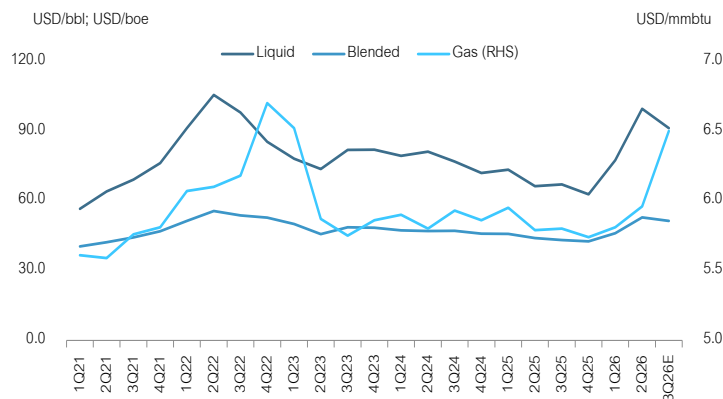
Fig 3: Quarterly estimated ASP (blended, liquid, gas)
