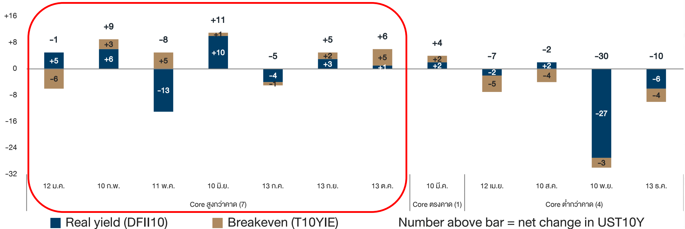
CPI days 2022: 10Y yield move split into real yield and breakeven
