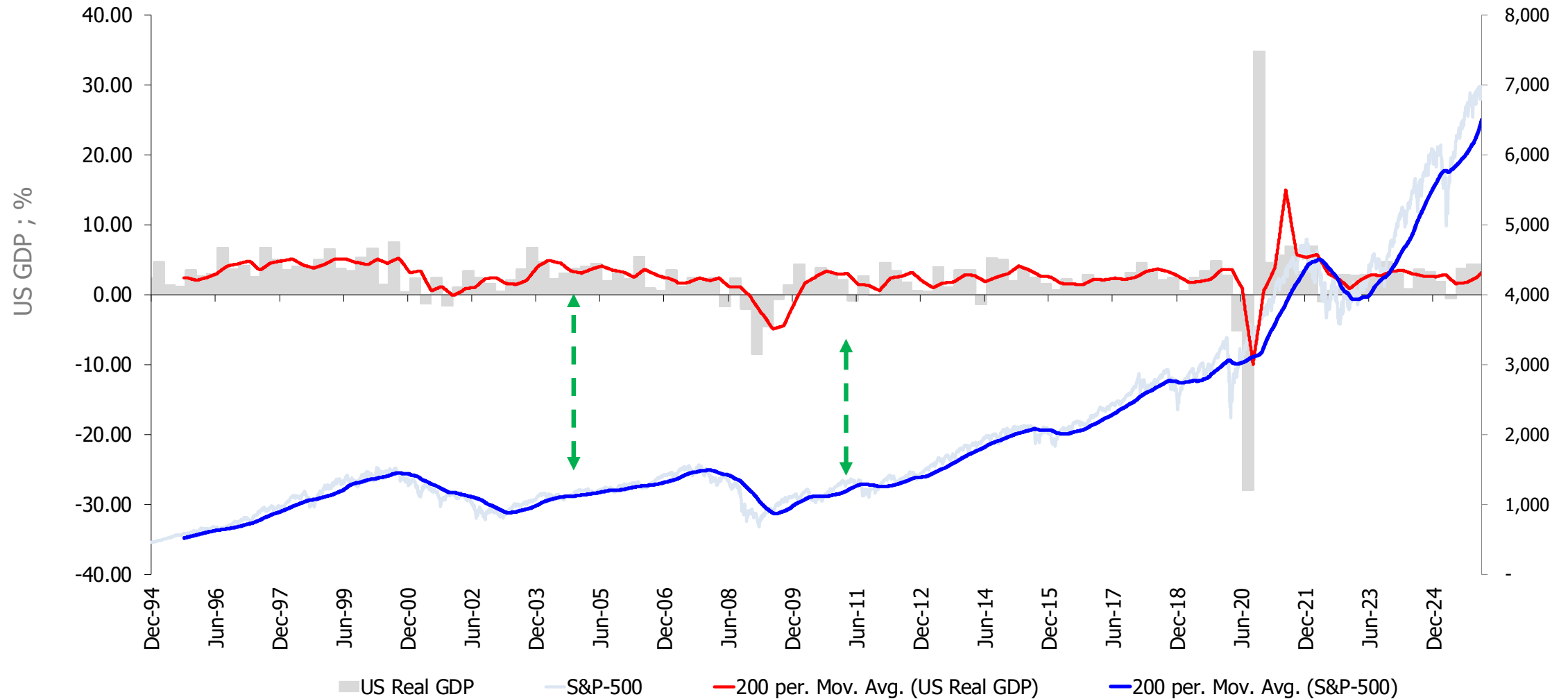
US Real GDP and S&P-500
